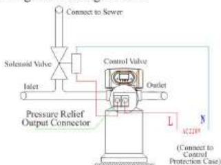
Figure 3-10 Wiring of Pressure Relief Output
