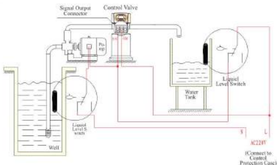
Figure 3-5 Wiring of Liquid Level Controller Controls Inlet Pump
