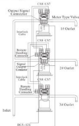
Figure 3-13 Series system
