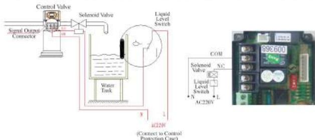
Figure3-1 Wiring of Solenoid Valve on Outlet
