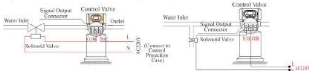
Figure 3-2 Wiring of Solenoid Valve on Inlet
