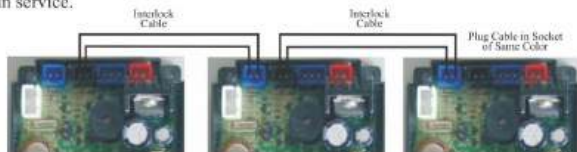
Figure 3-9 Network System Wiring with Interlock Cable
