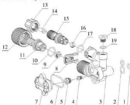
Structure Chart of New Injector:
