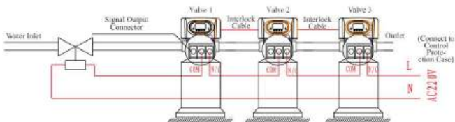
Figure 3-4 Wiring of Solenoid Valve in Inlet
