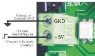
Figure 3-11 Wiring of Remote Input
