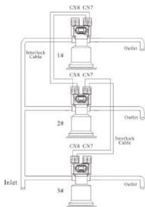
Figure 3-12 Interlock system
