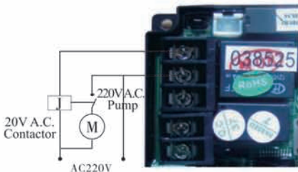
Figure 3-8 Wiring of Booster Pump on Inlet
