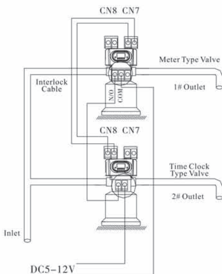
Figure 3-13 Series system
