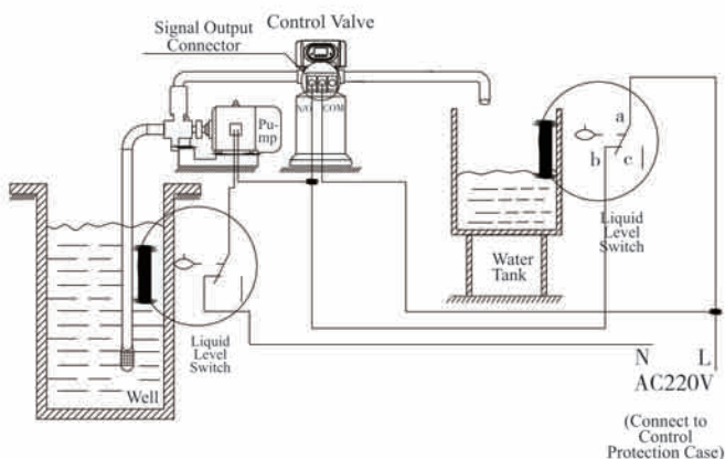
Figure 3-5 Wiring of Liquid Level Controller Controls Inlet Pump
