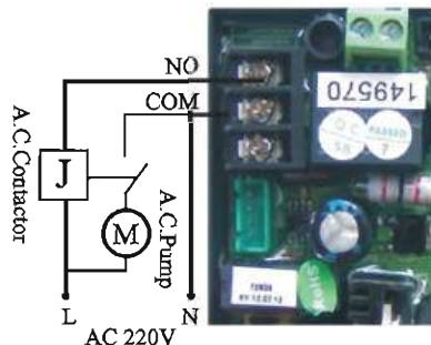
Figure12 Wiring of Booster Pump on Inlet Figure 13 Wiring of Booster Pump on Inlet
